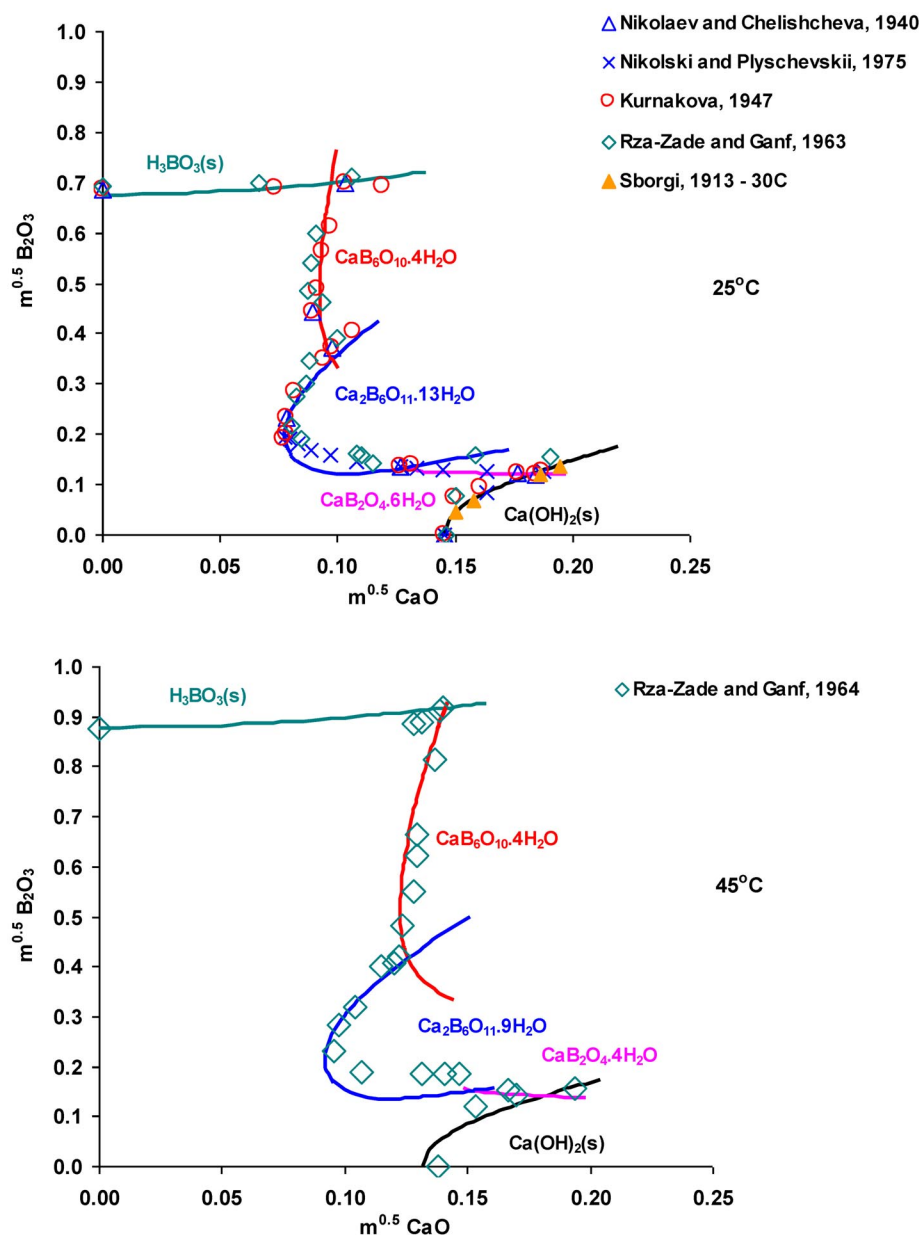
Fig. 10 Solubilities in the CaO + B 2 O 3 + H 2 O system at 25 and 45 °C. The symbols are literature data, and the lines are calculated using the MSE model.
