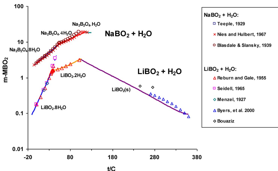
Fig. 5 Solubilities in the \text{NaBO}_2 + \text{H}_2\text{O} and \text{LiBO}_2 + \text{H}_2\text{O} systems. The symbols denote literature data, and the lines are calculated using the MSE model.
